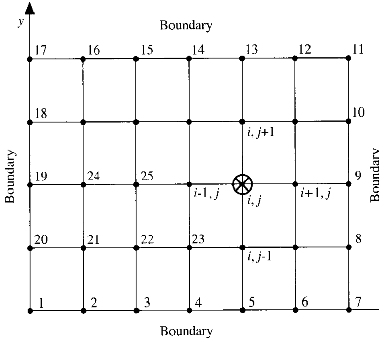
FIG. 6.4 Schematic for relaxation technique.
