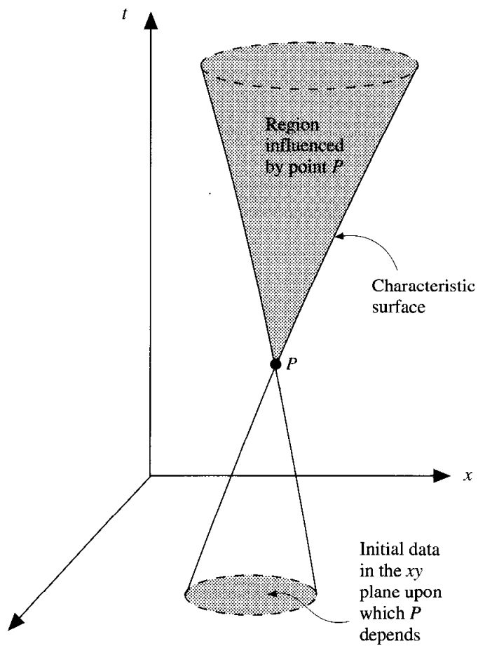
FIG. 3.7 Domain and boundaries for the solution of hyperbolic equations. Two-dimensional unsteady flow.
