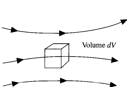
Infinitesimal fluid element fixed in space with the fluid moving through it
