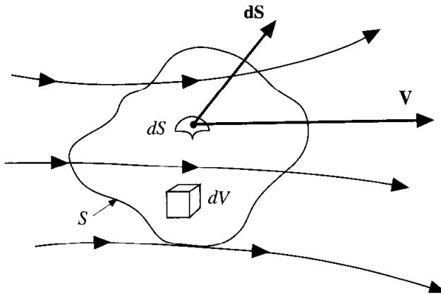
FIG. 2.5 Finite control volume fixed in space.
